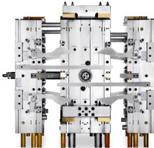
Stack Mold
