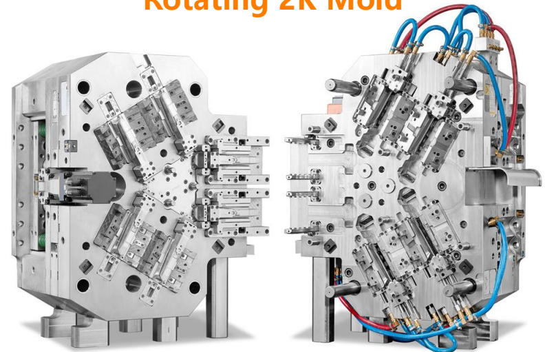
Rotating 2K Mold
