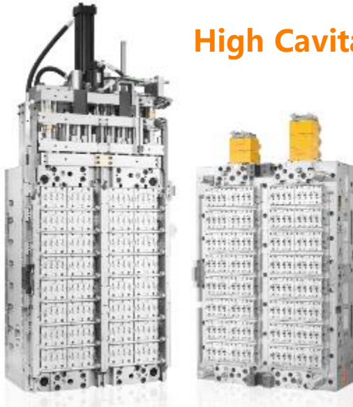
Stack Mold
